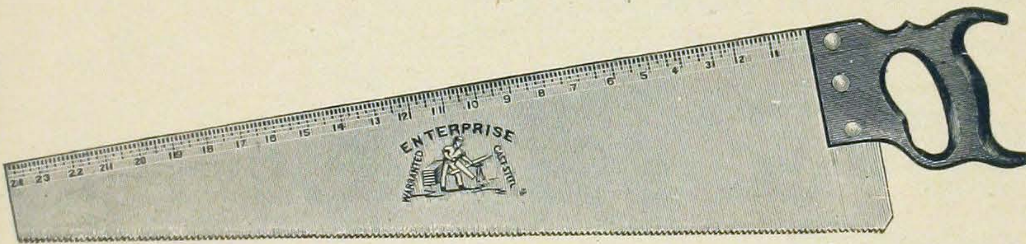
Beech Handle, Polished Edge, 3 Plain Screws, set and sharpened, 24 inch etched Rule.
